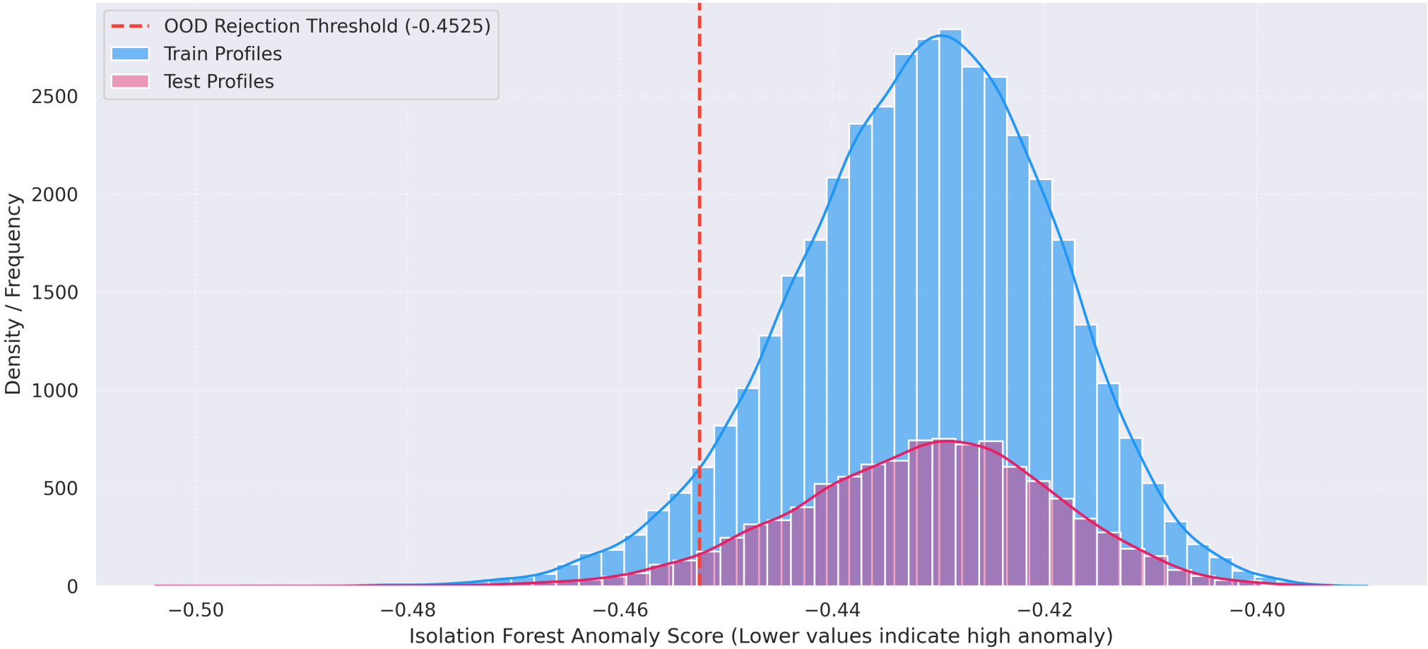
📊 OOD Rejection System: Profile Anomaly Score Distributions
