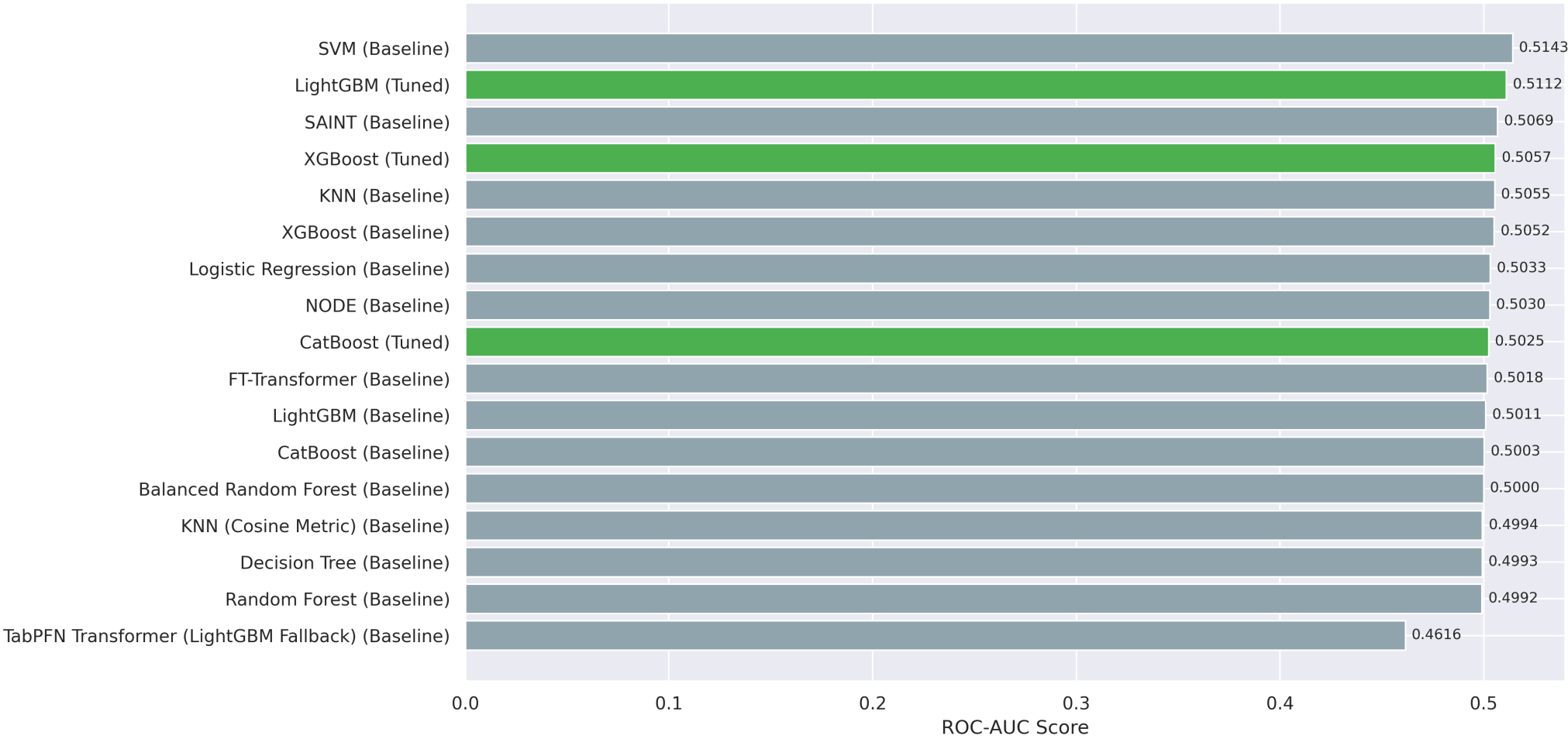
All Models Ranked by ROC-AUC Score (Green = Tuned, Gray = Baseline)
